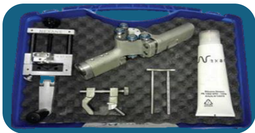
Terminating Tool
